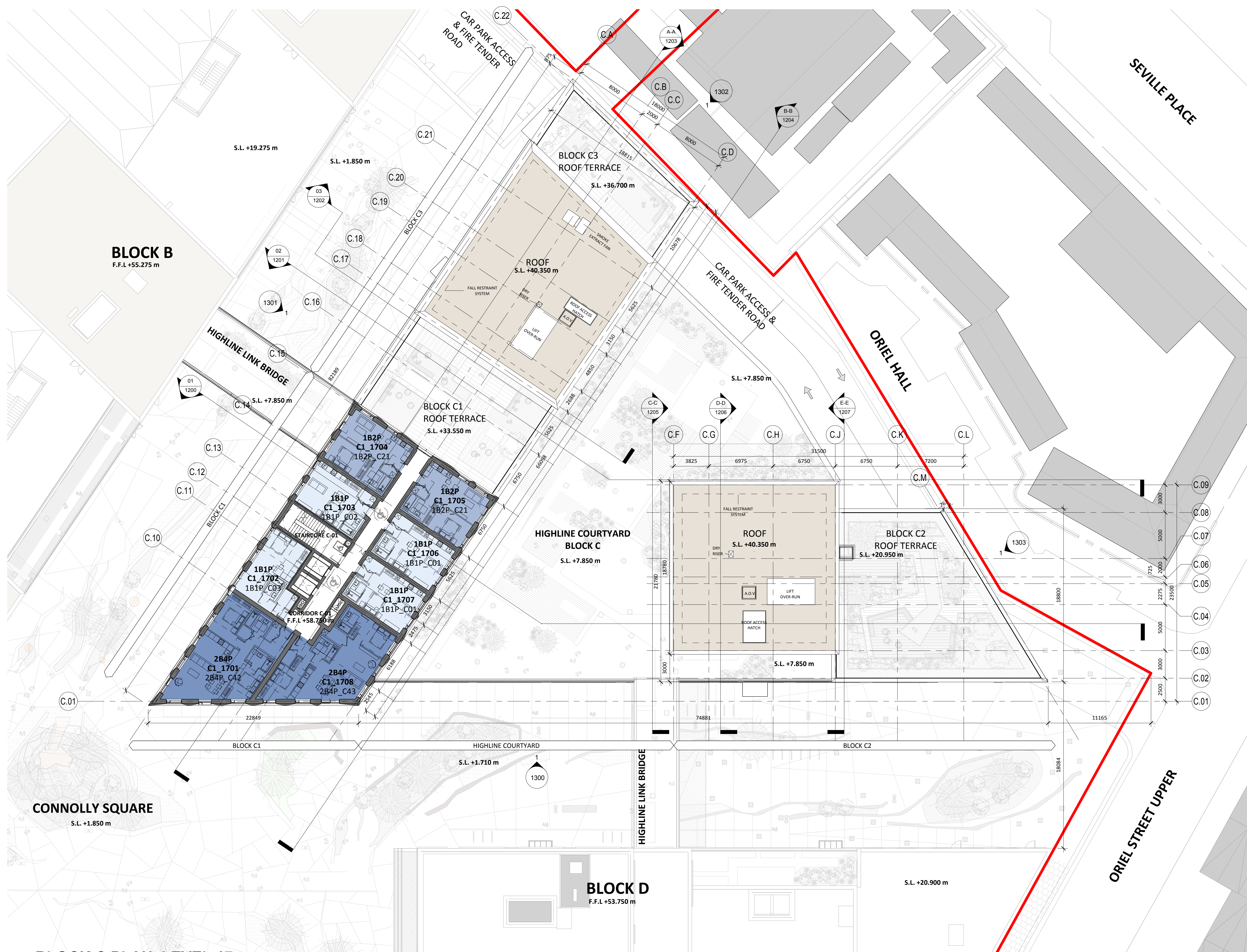
1 BLOCK C PLAN_LEVEL 17 1 : 200
